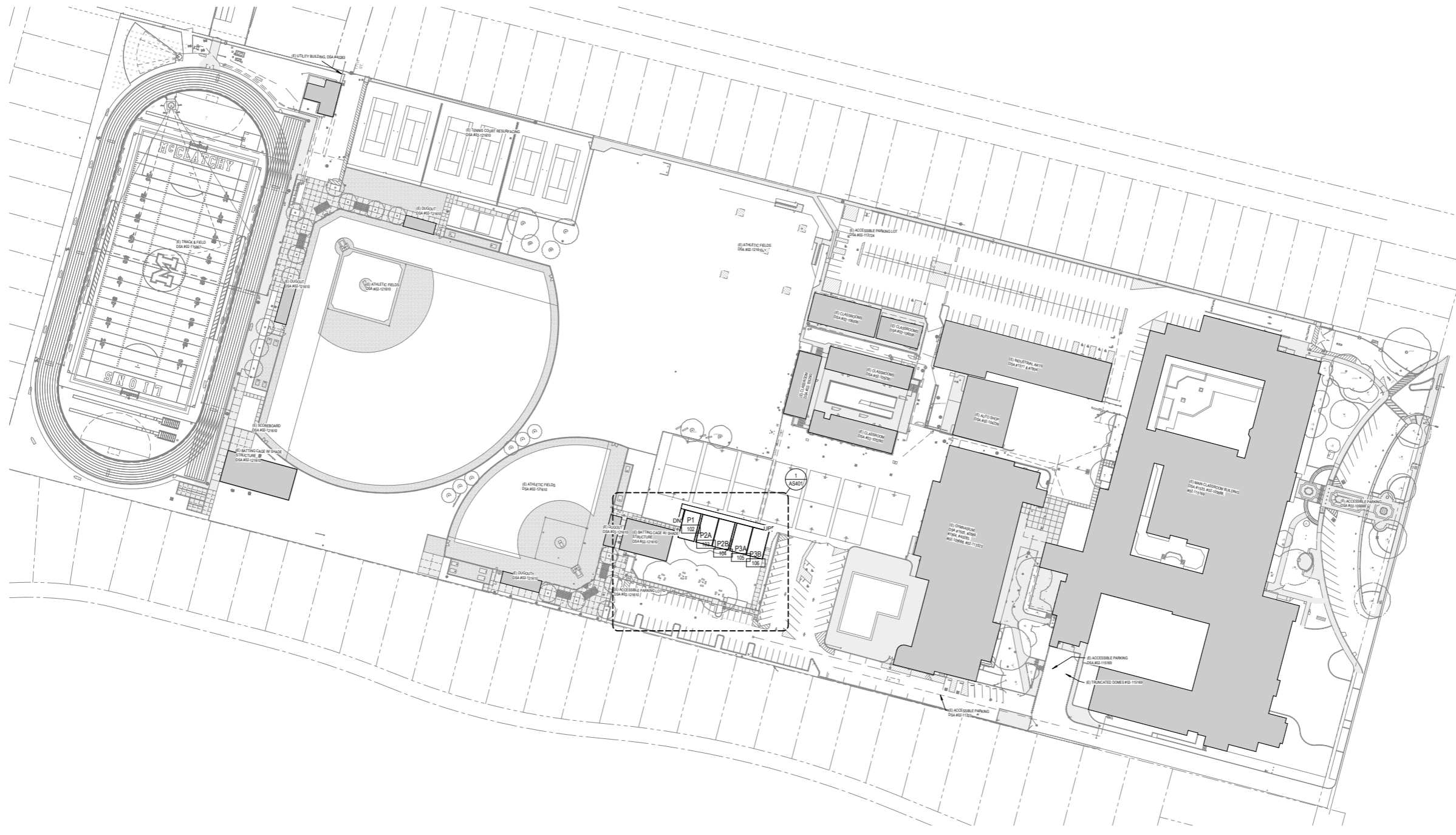
1 OVERALL SITE PLAN SCALE 1" = 60'-0"
