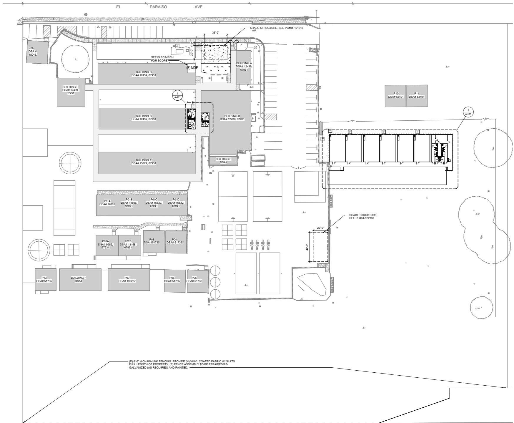
1 SITE PLAN - OVERALL SCALE 1" = 30'-0"
